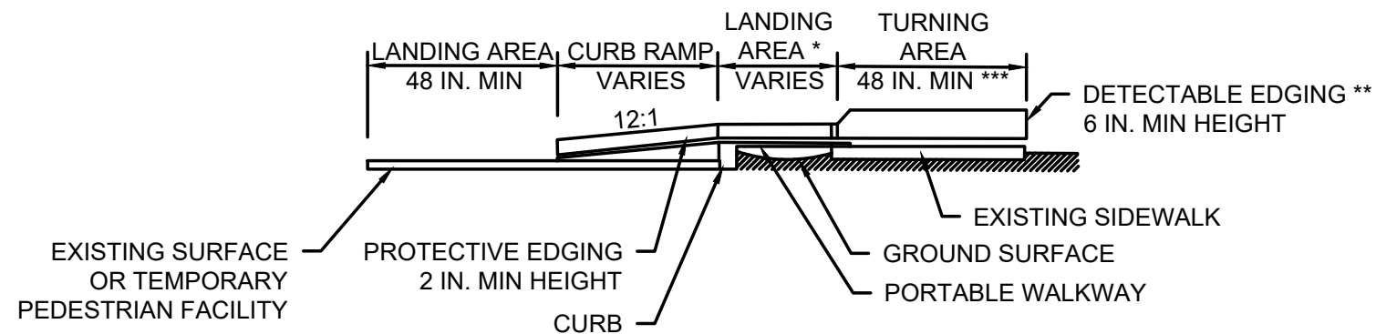
TEMPORARY CURB RAMP
