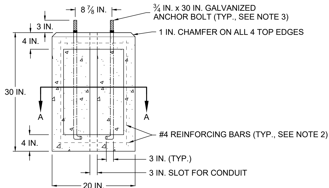
ELEVATION VIEW
