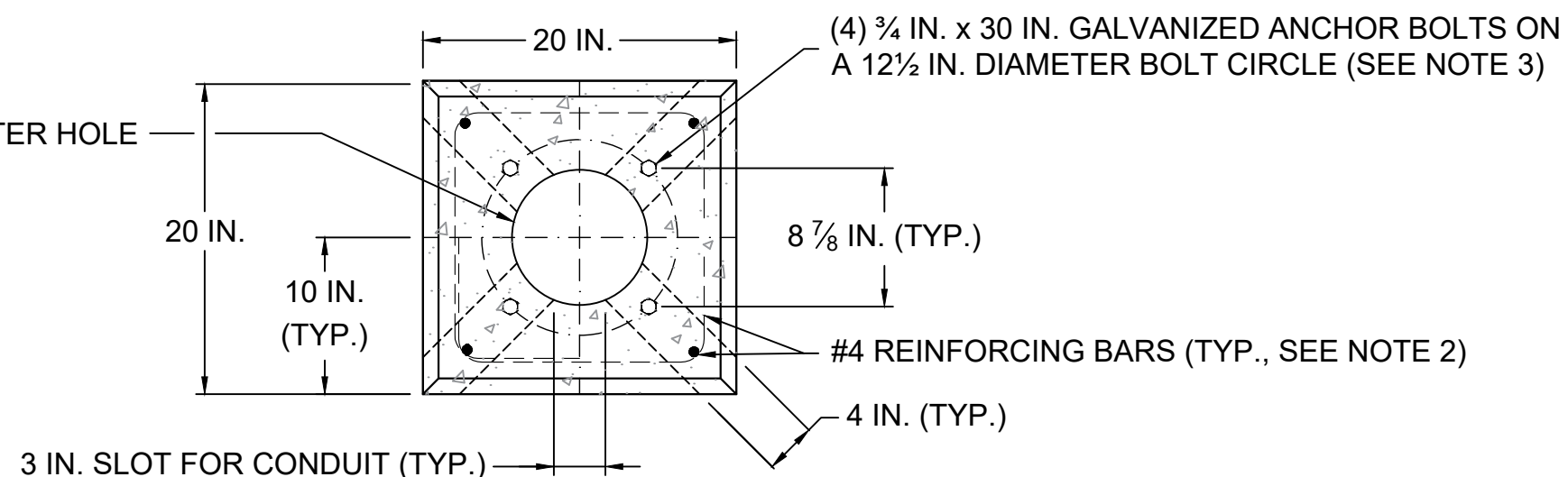
PLAN VIEW
