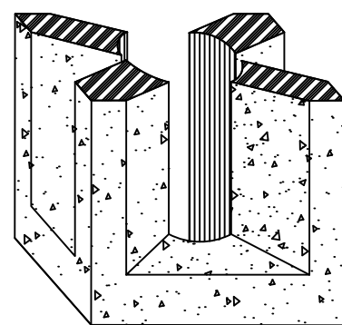
PICTORIAL VIEW (SECTION A-A)
