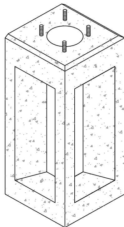
ISOMETRIC VIEW
