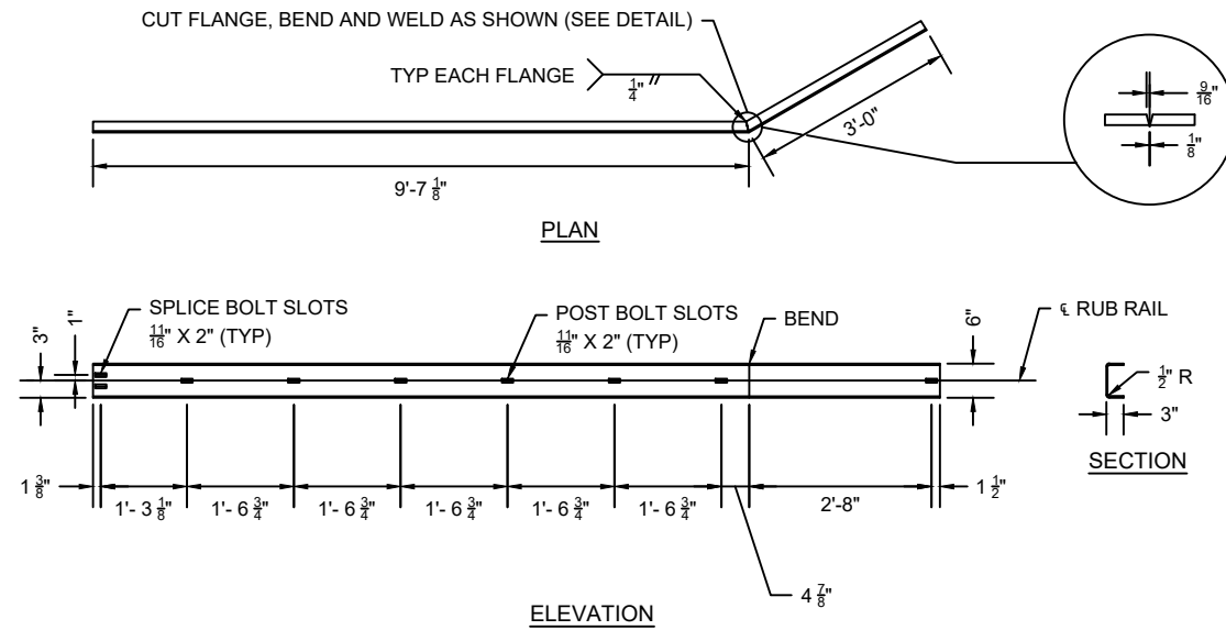
C6 X 8.2 RUB RAIL
