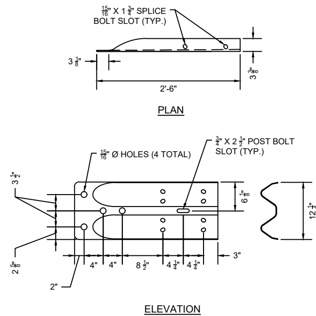
TERMINAL CONNECTOR
