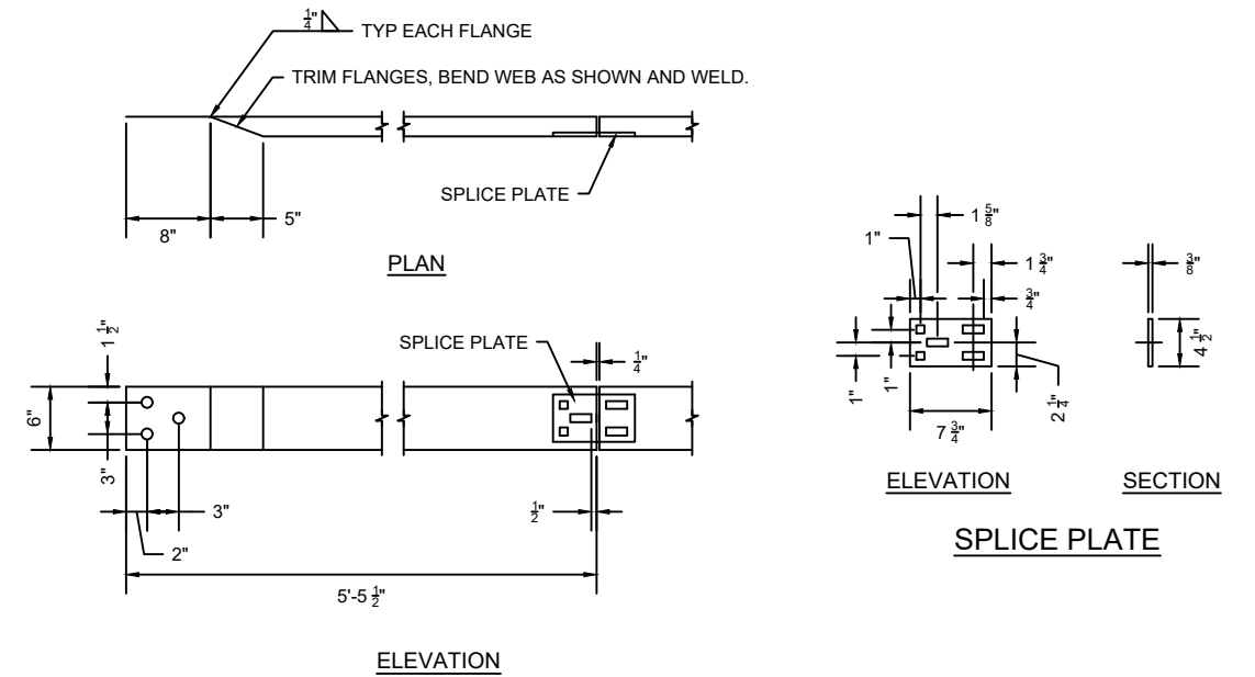
RUB RAIL - END DETAIL
