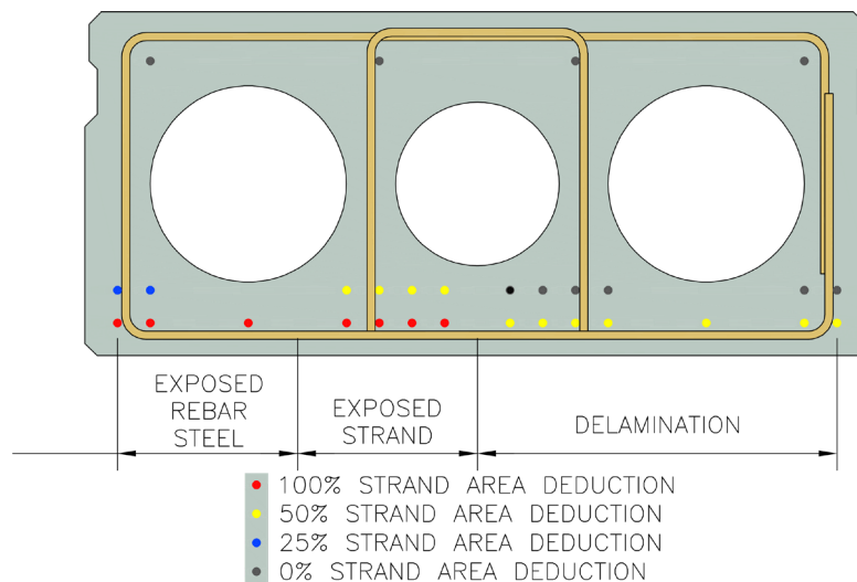
Figure 7.2.10-2: Deck Beam Cross-Section (see Figure 7.2.10-1)
