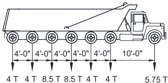
Figure 7.5.2-11: Vehicle Diagrams – Specialized Hauling Vehicles
